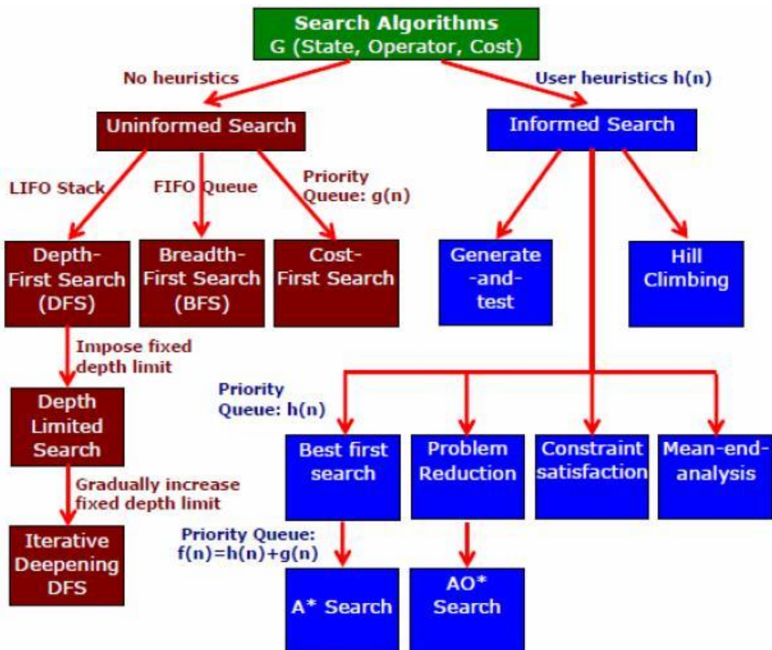
Fig. Different Search Algorithms
